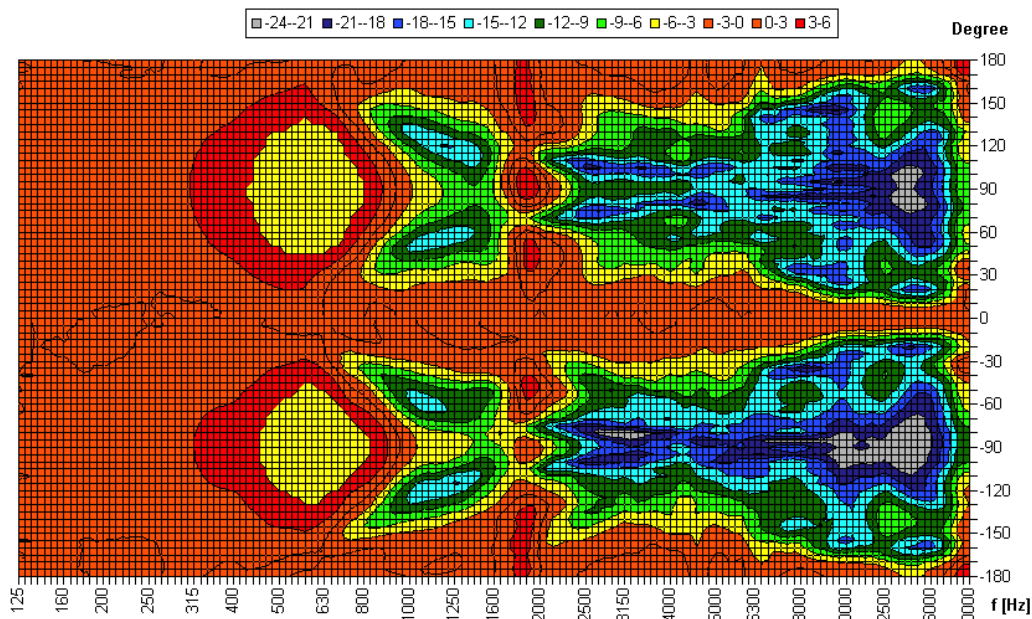
Horizontal Isobars of: Elko-Schmid Lamprodyn-130-bi-DC
