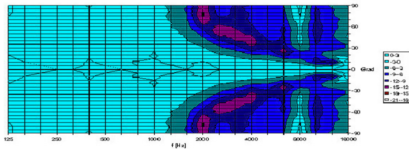
2D Directivity Plot
