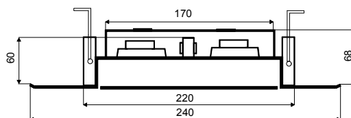
SLB-240-AB WITH 68-MM-FIREDDOME
