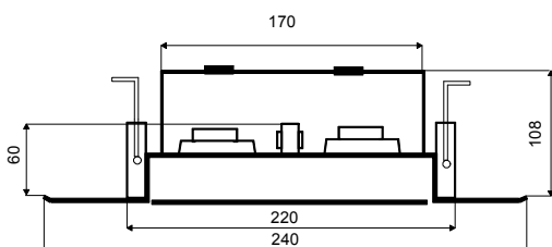
SLB-240-AB WITH 108-MM-FIREDDOME
